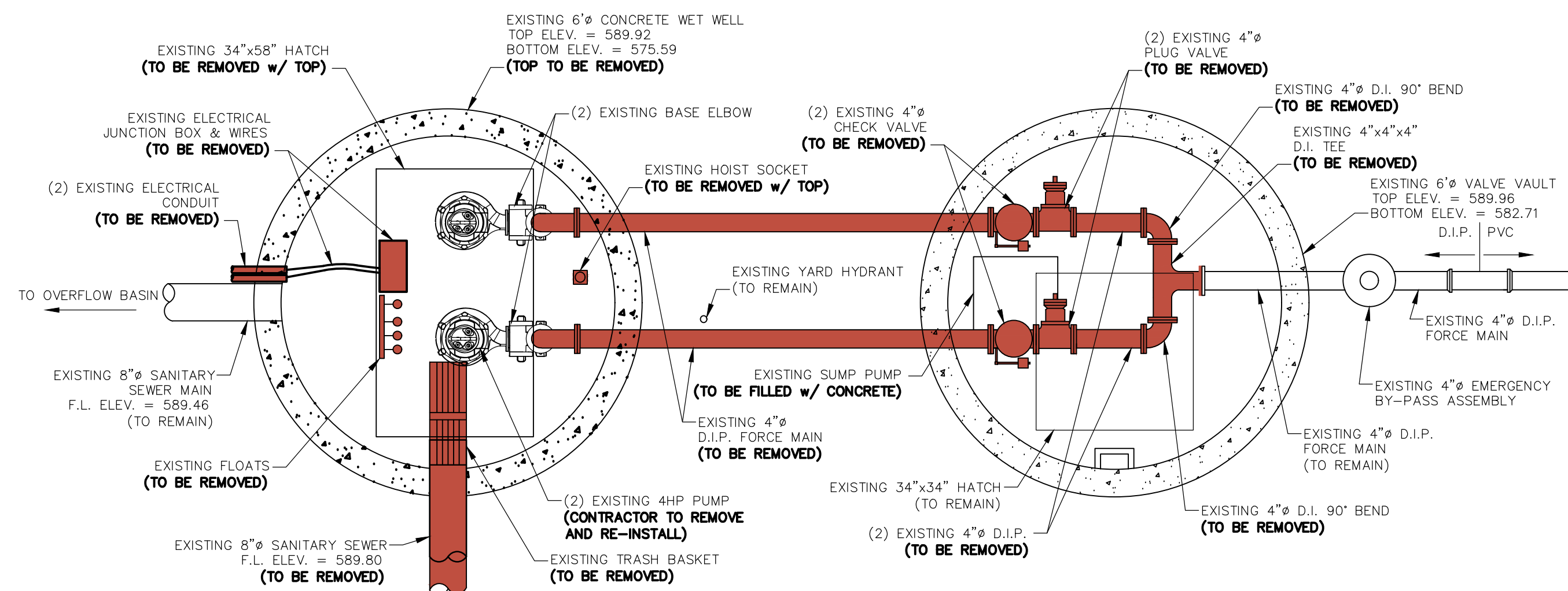
LIFT STATION PLAN VIEW SCALE: 1" = 2'
