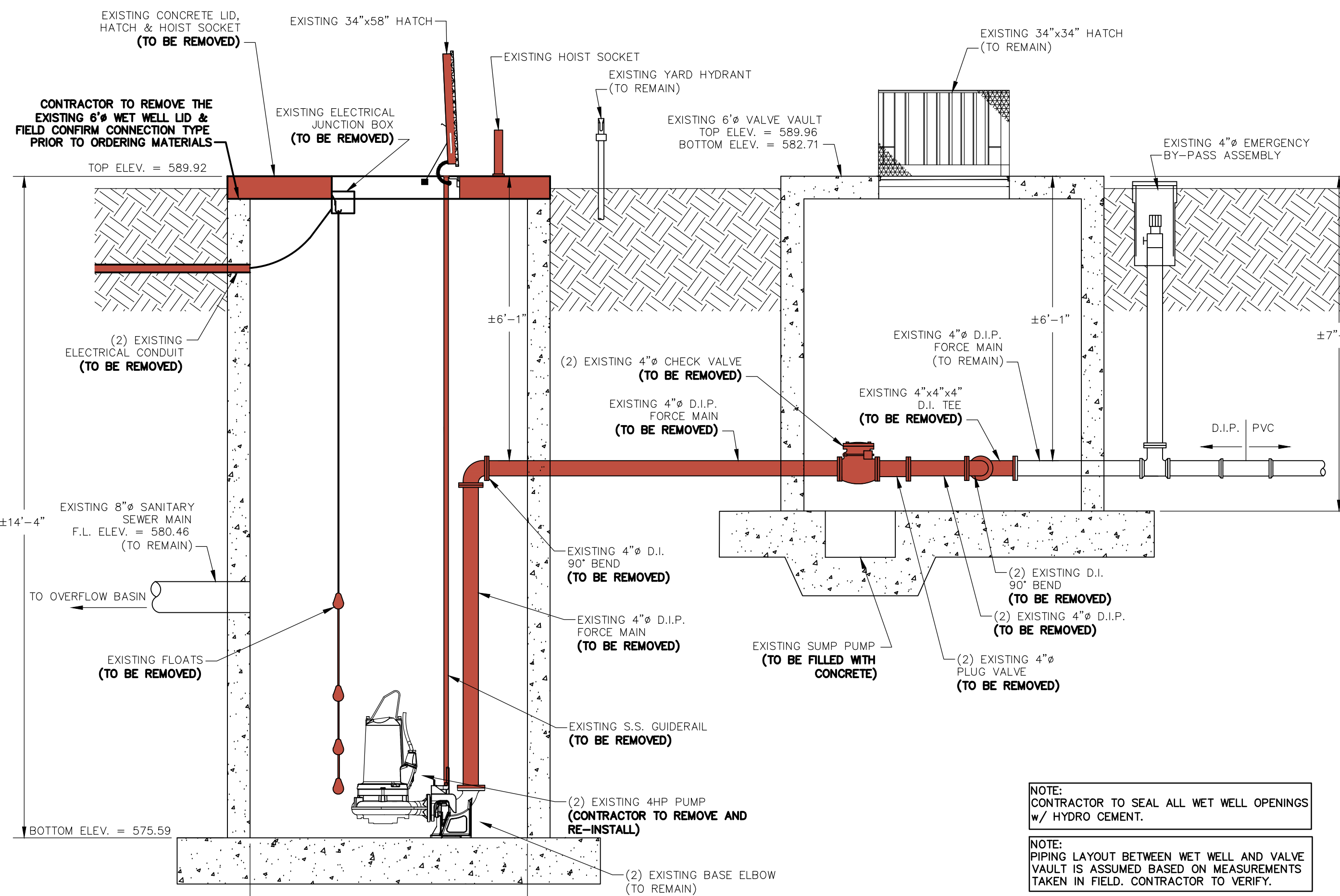
LIFT STATION PROFILE VIEW SCALE: 1" = 2'
