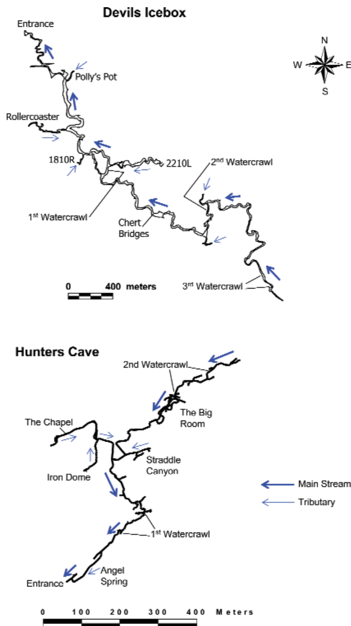
Figure 2. Line plot diagrams of the two cave systems. (Note the difference in scale for the two caves.)
